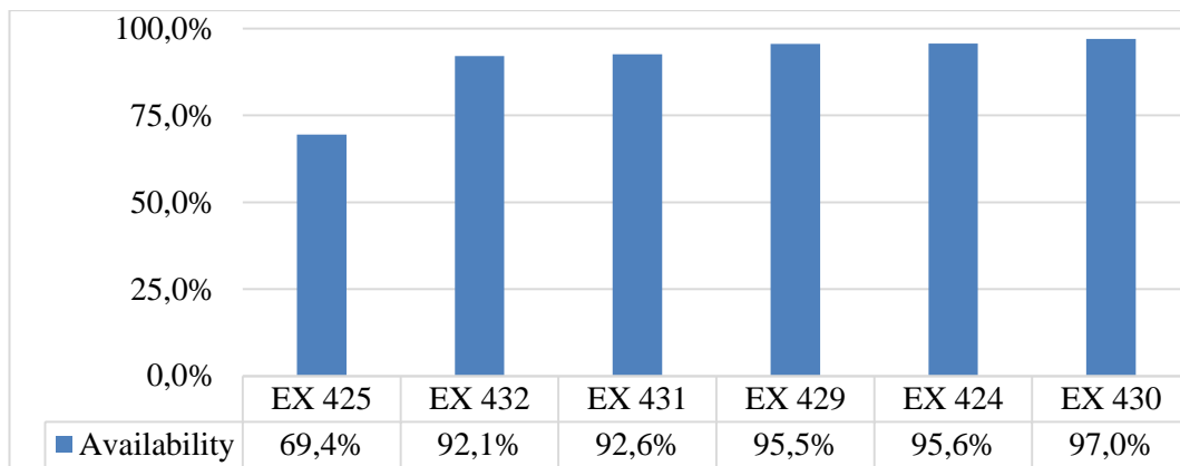
Gambar 1. Availability All Excavator
