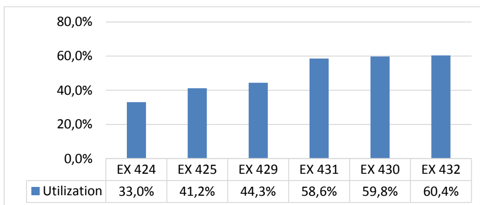
Gambar 2. Utilization All Excavator
