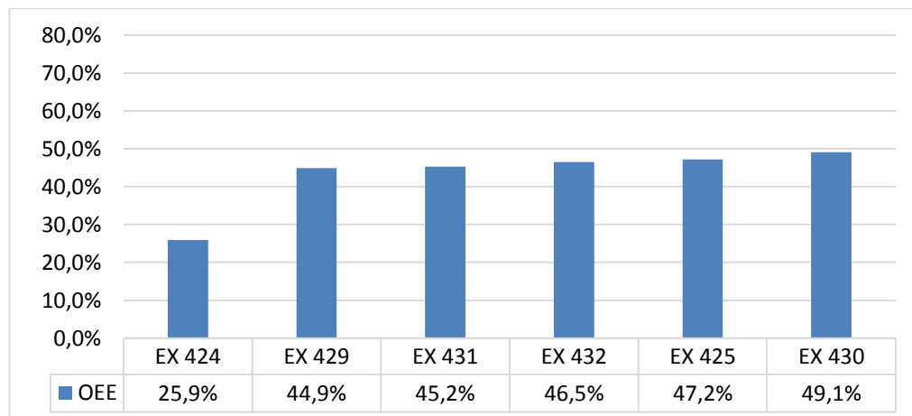
Gambar 4. Nilai OEE All Excavator
