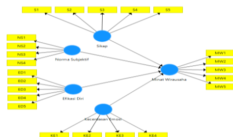
Gambar 1. Framework penelitian
