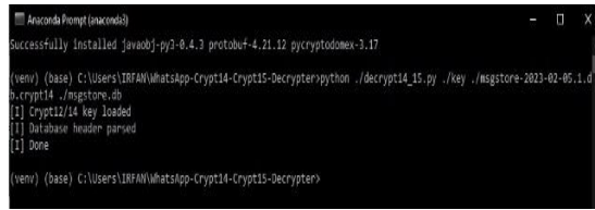
Gambar 8. Proses decrypt
