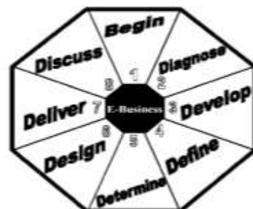
Gambar 2. Metode Overview
