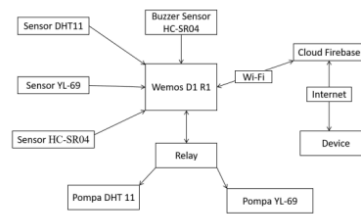
Gambar 3. Deployment Diagram
