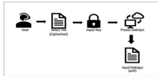
Gambar 9. Proses dekripsi
