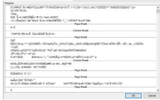
Gambar 8. Ciphertext preview
