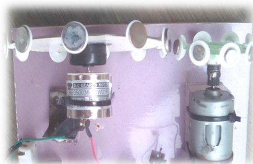
Gambar 16. Generator Turbin Magnet.
