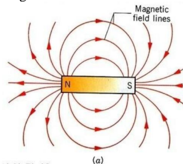
Gambar 1. Sumbu Magnet Sumber: Suyoso, 2003.
