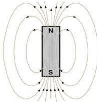
Gambar 3. Fluks Medan Magnet Sumber: Suyoso, 2003.
