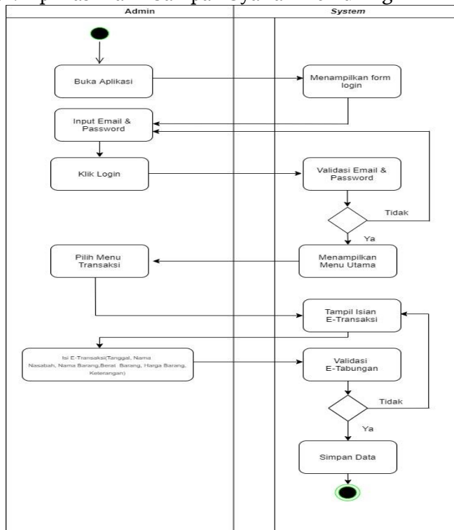
Gambar 5 Activity Diagram Transaksi Penimbangan Sampah
