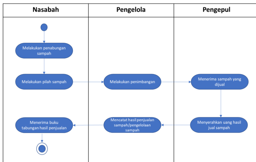
Gambar 2 Activity Diagram Sistem Berjalan
