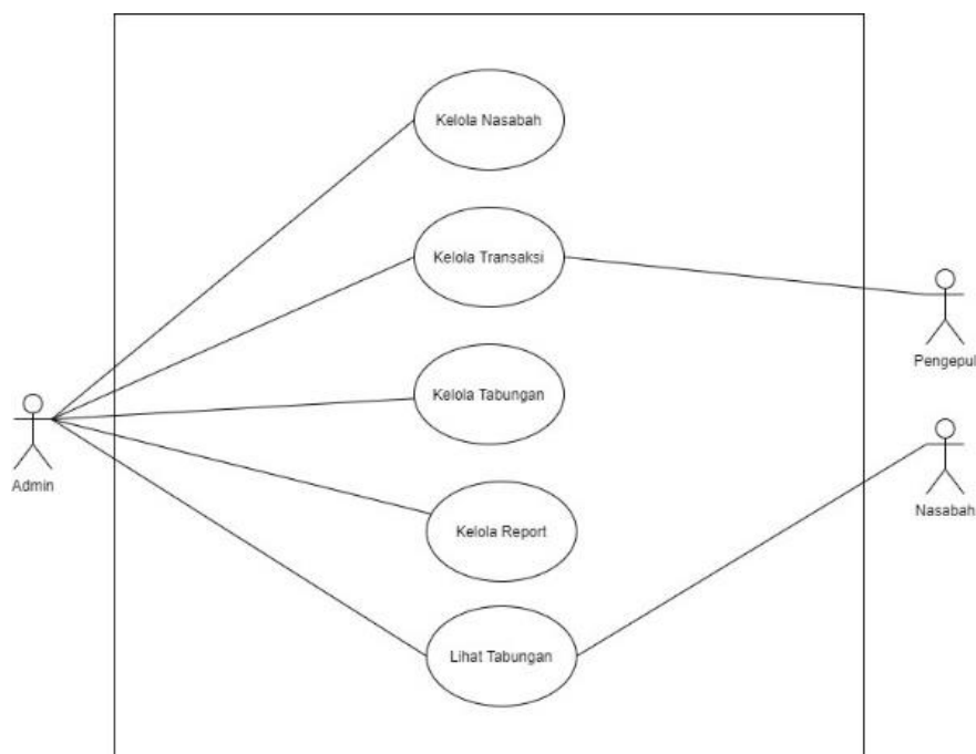
Gambar 3 Use Case Diagram Sistem Berjalan
