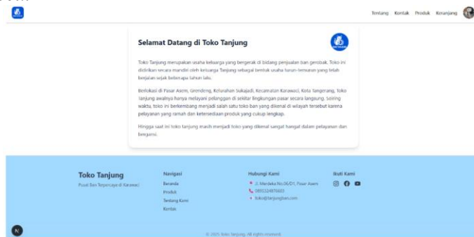
Gambar 9 Halaman About
