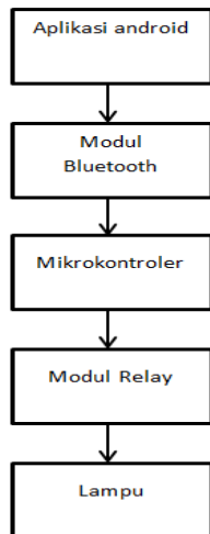
Gambar 3.2 Diagram blok system
