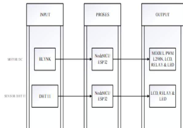
Gambar 1 Blok diagram
