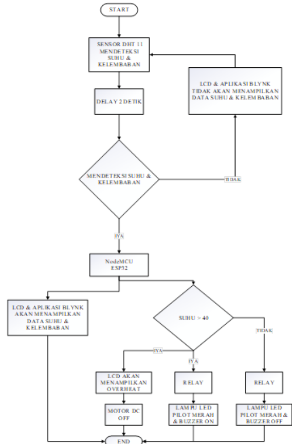
Gambar 3 Flowchart Sistem Kontrol DHT11
