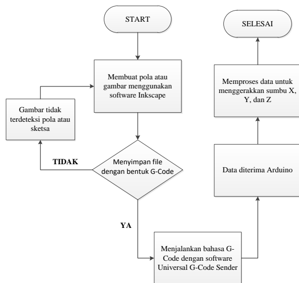
Gambar 2. Flowchart
