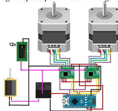
Gambar 3. Wiring diagram
